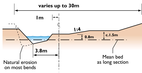
SECTION B THROUGH ASYMMETRICAL CHANNEL
