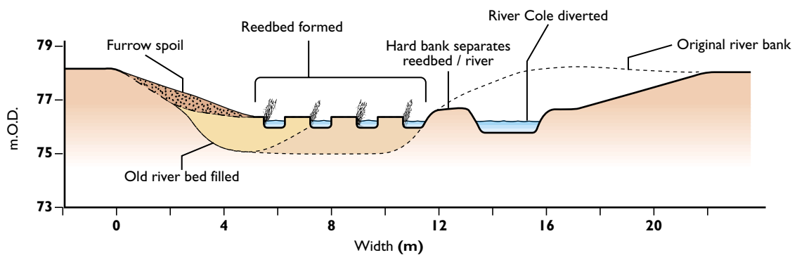
Figure 9.2.2 SECTION A – A
